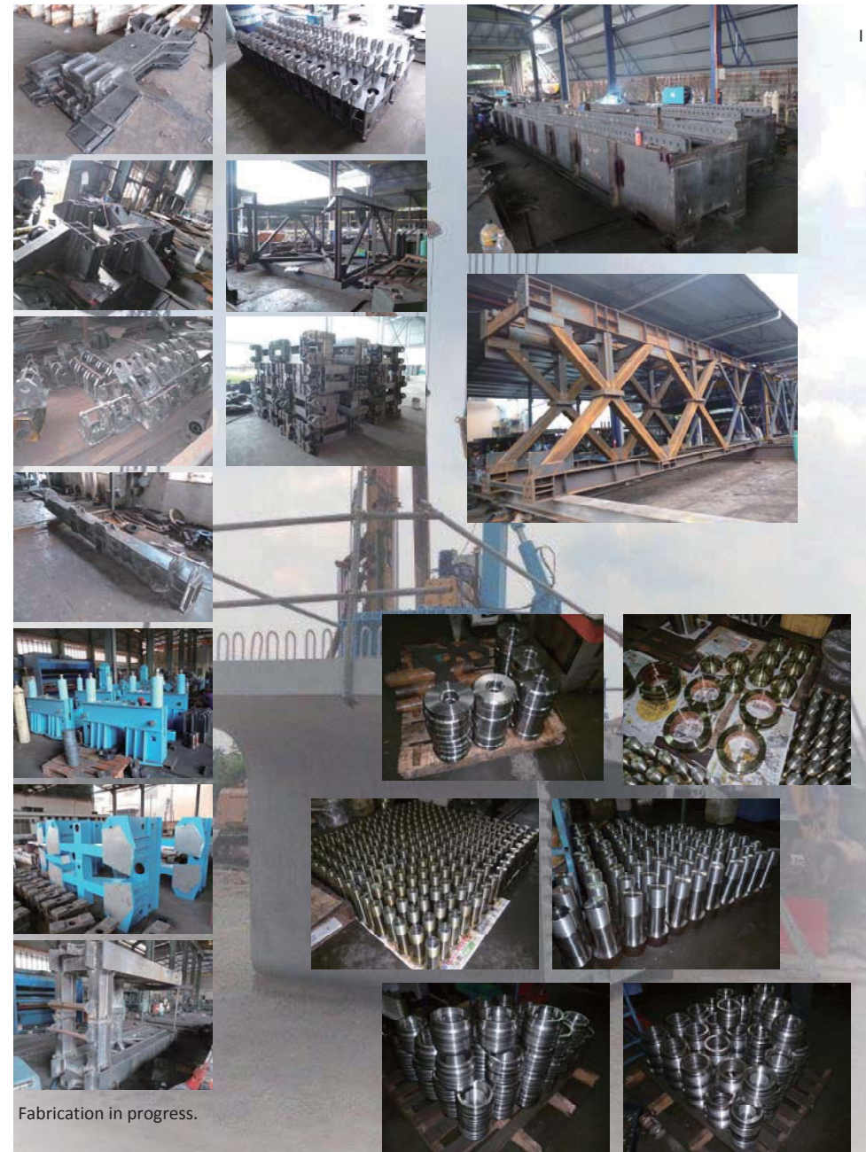
Machining Items.
