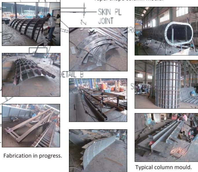
Taper shape column mould.
